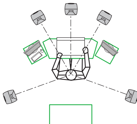
Figure 4. Symmetrical layout and keeping the acoustic axis clear from obstructions minimizes reflection surfaces and maintains accurate localisation because reflections are symmetrical.
