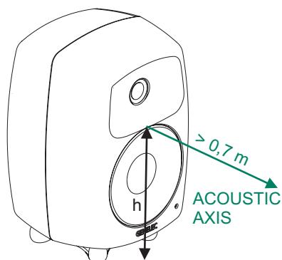
Figure 3. The location of the acoustic axis is on the center-line of the monitor at the given height “h”.
