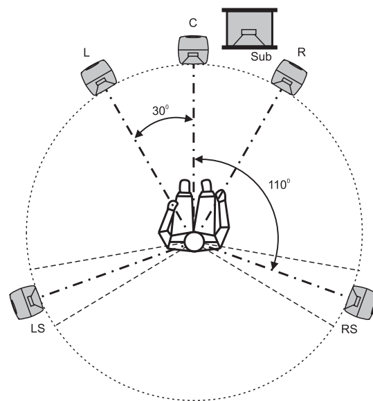
Figure 6. Recommended monitor positioning for 5.1 multi-channel audio reproduction
