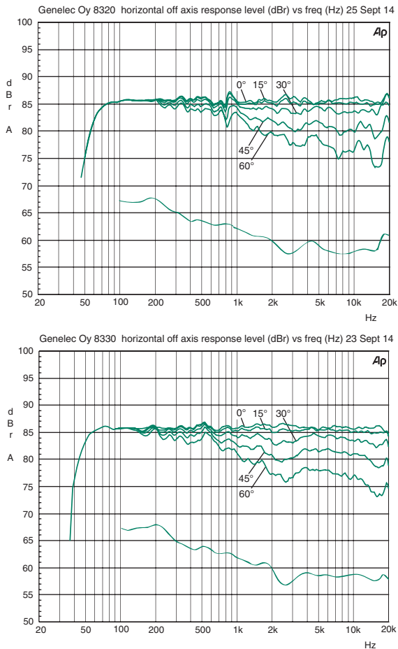
Figure 5: Frequency response plots in horizontal plane of the 8320A and 8330A. The lower curve is the monitor's power response.
