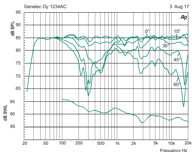
Figure 11. Horizontal directivity characteristics of the 1234AC (enclosure in horizontal configuration). The lower curve is the monitor's power response.
