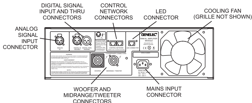
Figure 8. Connector panel of the RAM-XL amplifier.
