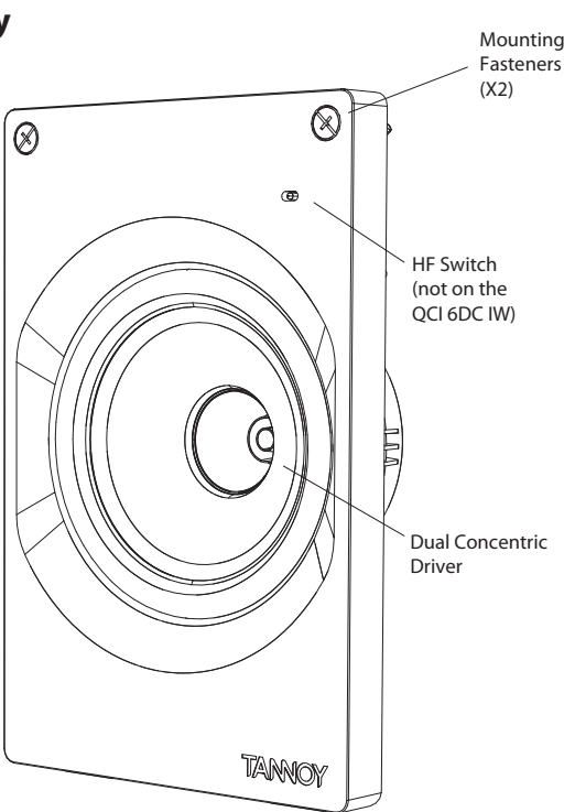
Speaker Assembly
