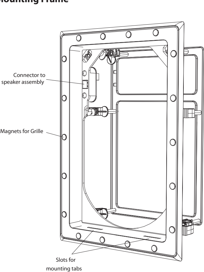
Mounting Frame
