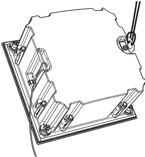
Fig. 16. Connecting the secondary safety to the back can
