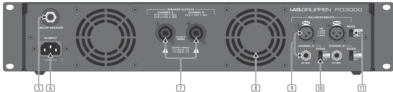
Fig. 2: Painel Traseiro do PD3000
