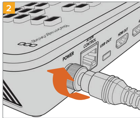
2 Secure the connector to ATEM Mini by tightening the connector screw
